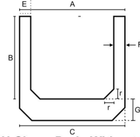
S.C U-Shape Drain Without DWF
