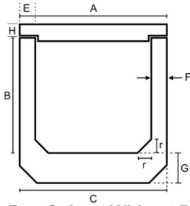
R.C. Box Culvert Without DWF
